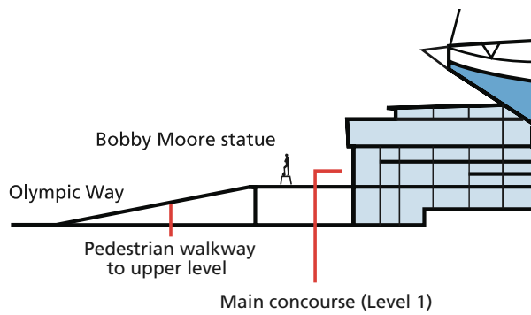
Section view of North side of the stadium
